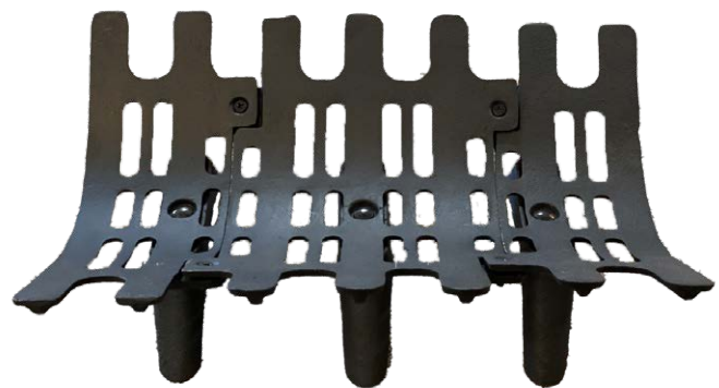
SFG-22 SELF FEEDING CAST IRON GRATE 22" LONG X 15 1/2" DEEP X 8" HIGH 3 1/2" CLEARANCE 3 LEGS: 11" LONG X 2" WIDE 33 LBS. MASTER PACK: 1 095192 206101
