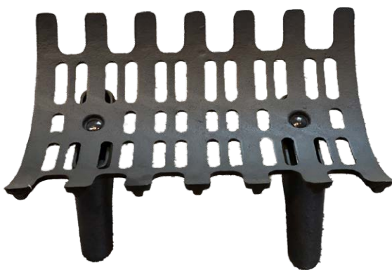
SFG-18 SELF FEEDING CAST IRON GRATE 17 1/2" LONG X 11 1/2" DEEP X 7" HIGH 3 1/2" CLEARANCE 2 LEGS: 11" LONG X 2" WIDE 21 LBS. MASTER PACK: 1 095192 206057
