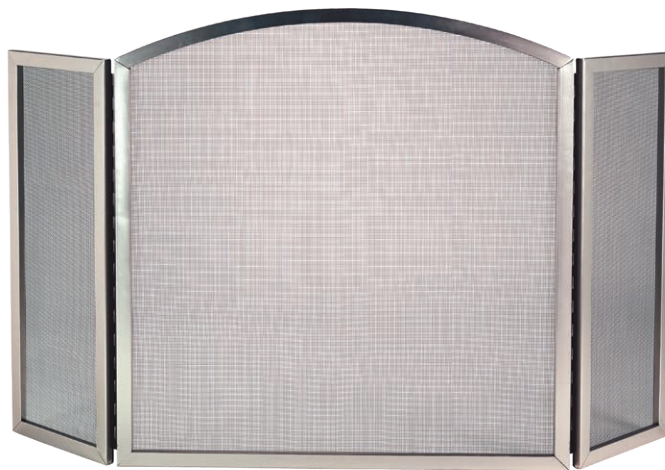
S702 3 FOLD ARCHED SATIN NICKEL SCREEN 31" HIGH X 50" WIDE 25 LBS. MASTER PACK: 2 095192 146155
